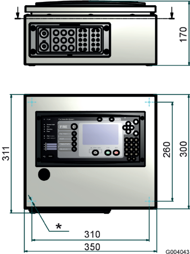
Figure 2. Wall mounting dimensions for Cabinet
